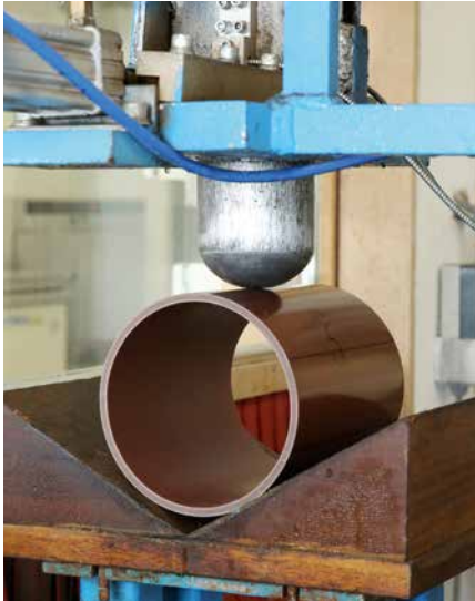
12,5 kg from a height of 2 m (-10 °C)
